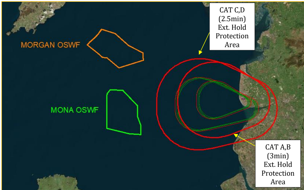
Figure 203 - Windfarms vs NDB(L) RWY 10 Extended Holdings
