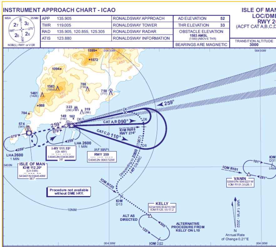
Figure 138 - LOC/DME RWY 26
