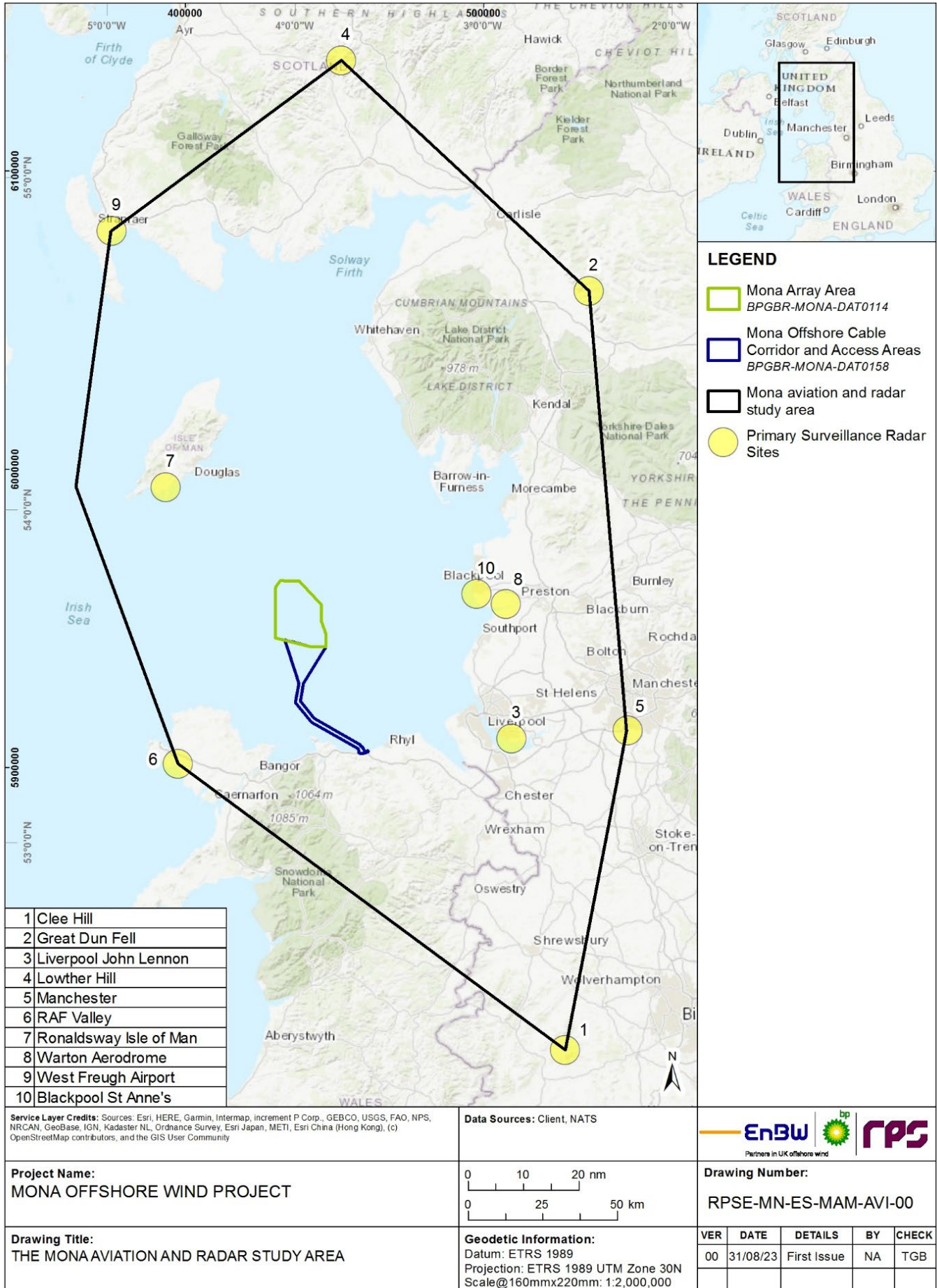
Figure 1.1: The Mona aviation and radar study area.
