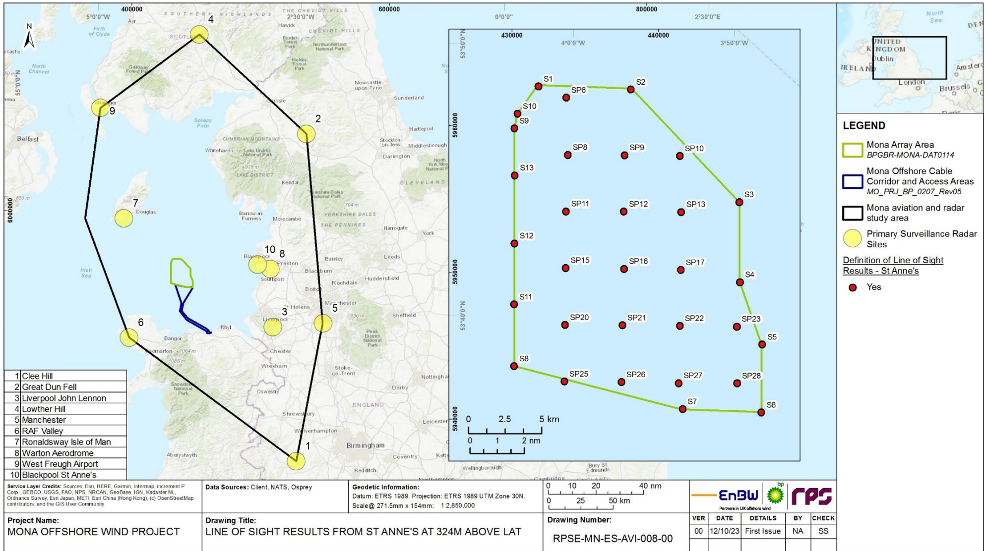
Figure 1.5: NATS St Anne's PSR LoS of the Mona Array Area (not to scale).
