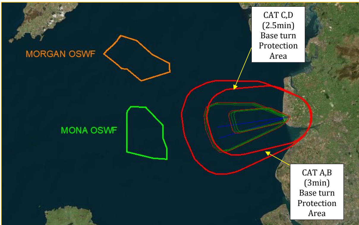
Figure 202 - Windfarms vs NDB(L) RWY 10 Base turns
