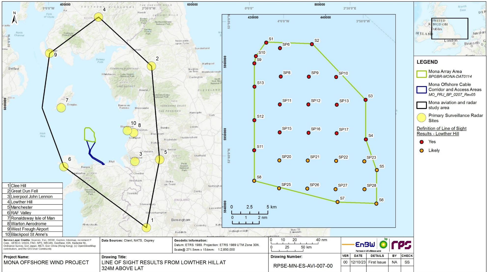
Figure 1.4: NATS Lowther Hill PSR LoS of the Mona Array Area (not to scale).
