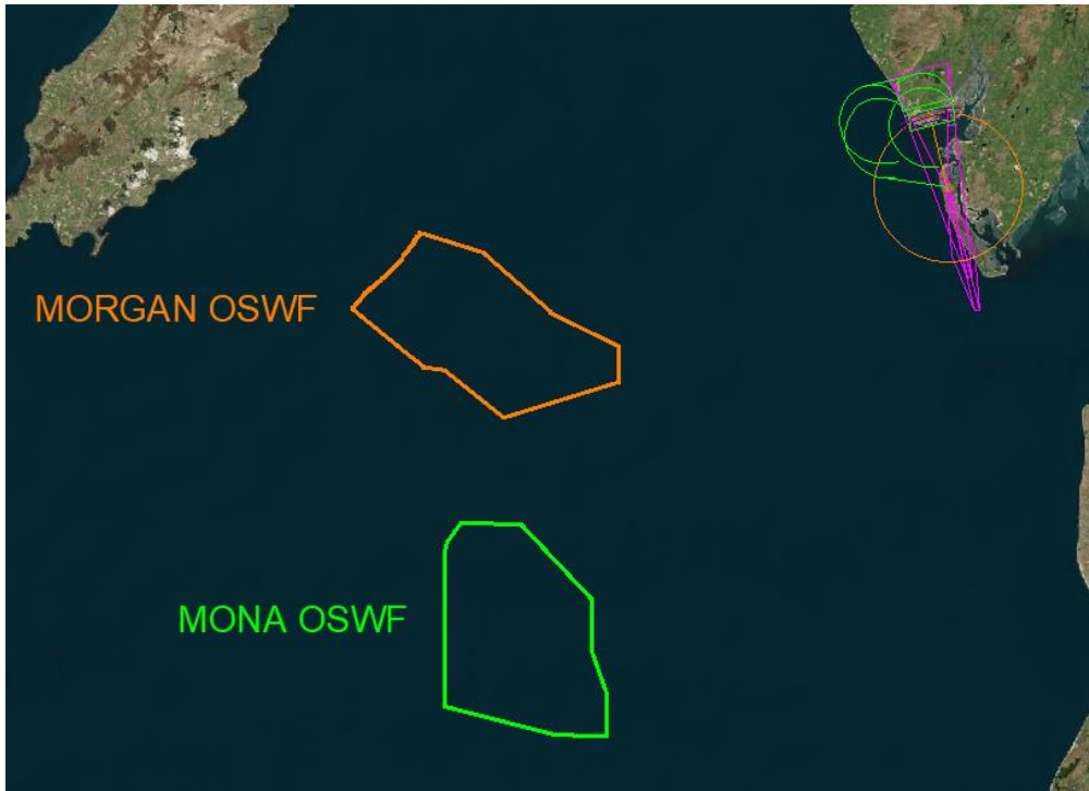
Figure 225 - Morgan and Mona Windfarm vs ILS/DME RWY 35 Protection Areas
