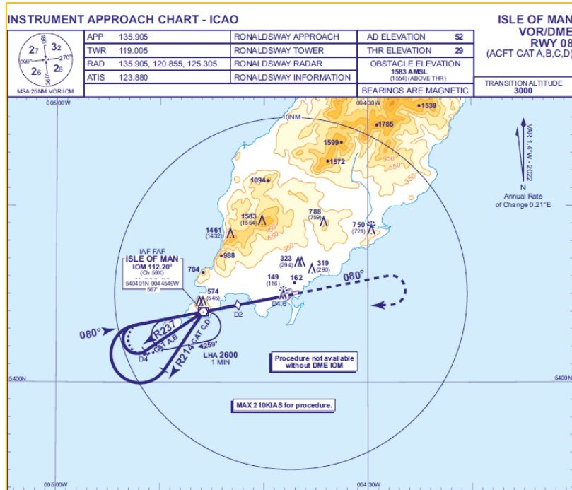
Figure 125 - VOR/DME RWY 08
