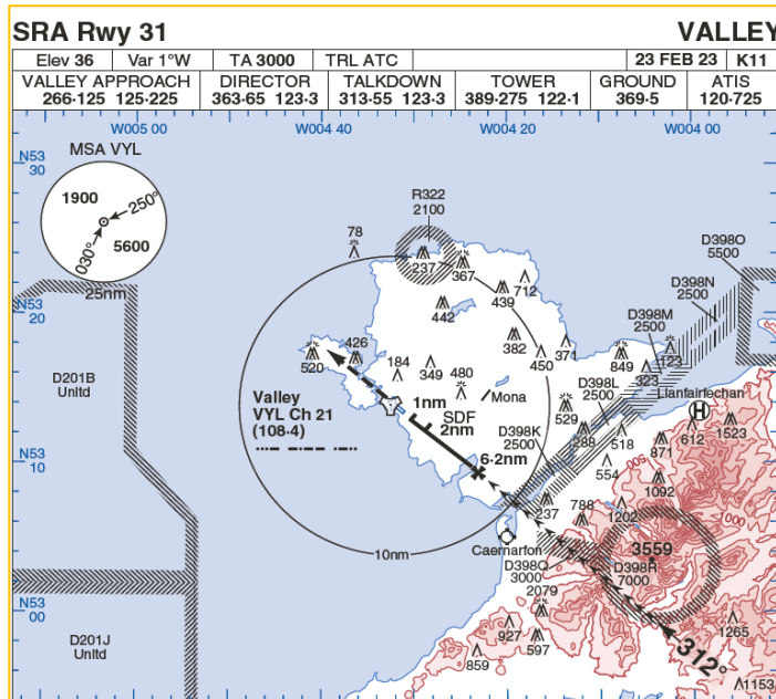
Figure 179 - SRA RWY 31 Procedure
