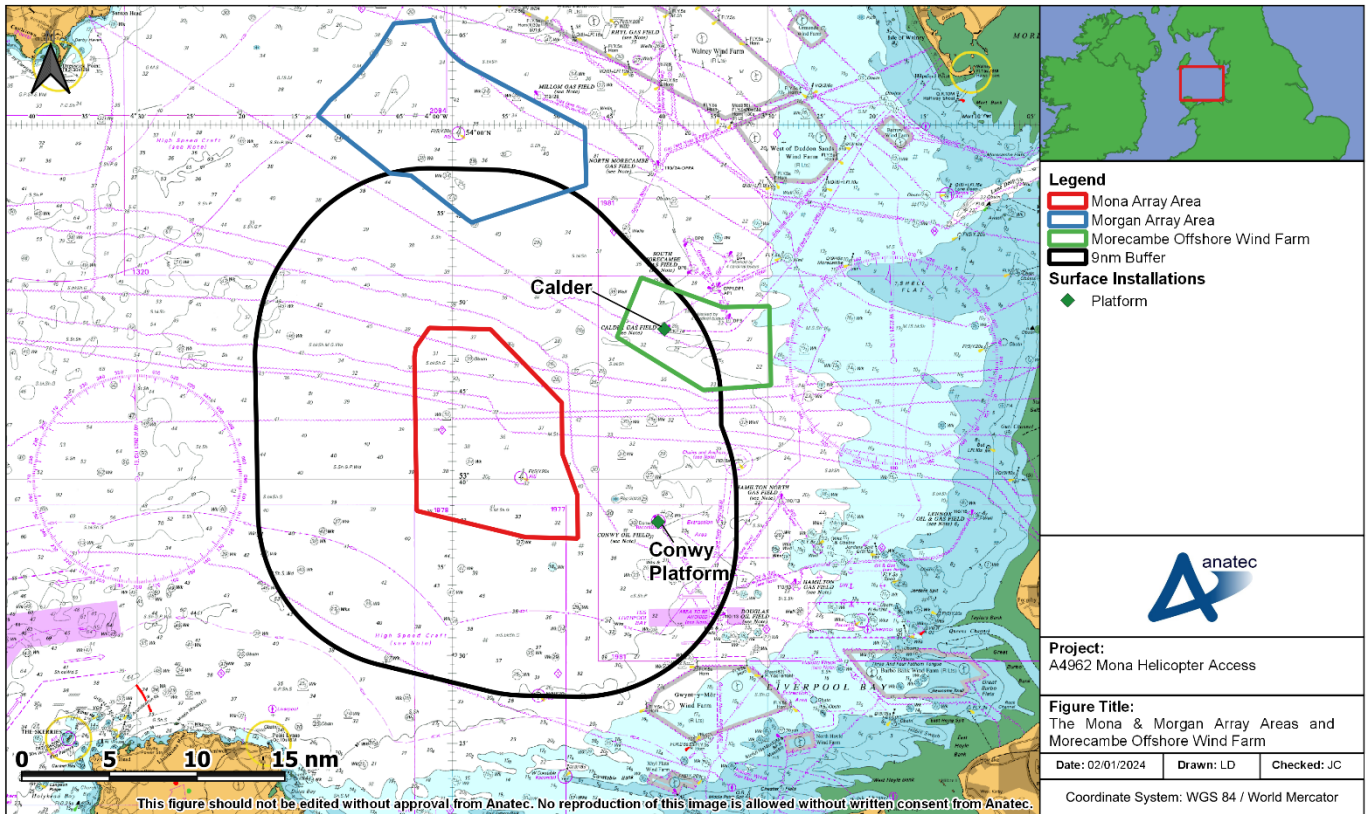
Figure A. 8: The Mona and Morgan Array Areas and Morecambe Offshore Windfarm.
