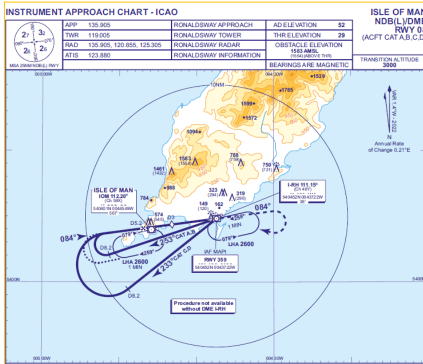
Figure 129 - NDB(L)/DME RWY 08
