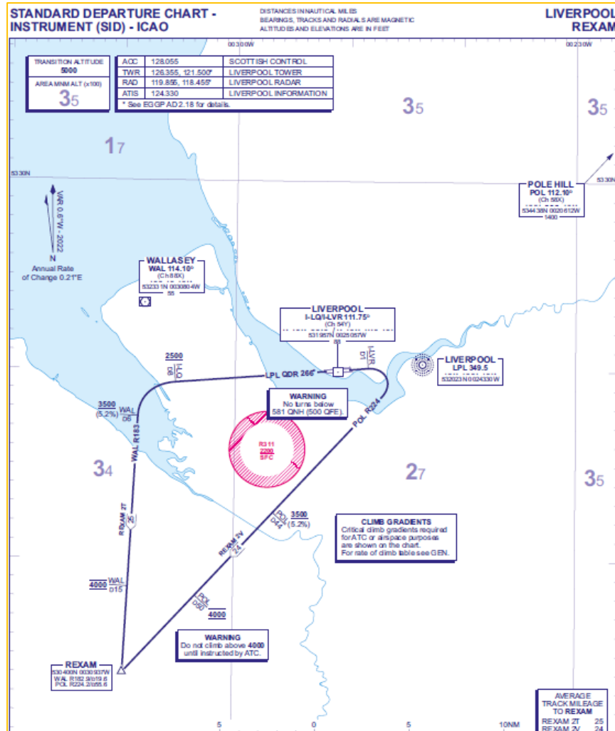
Figure 41 - SID REXAM 2V 2T Procedure
