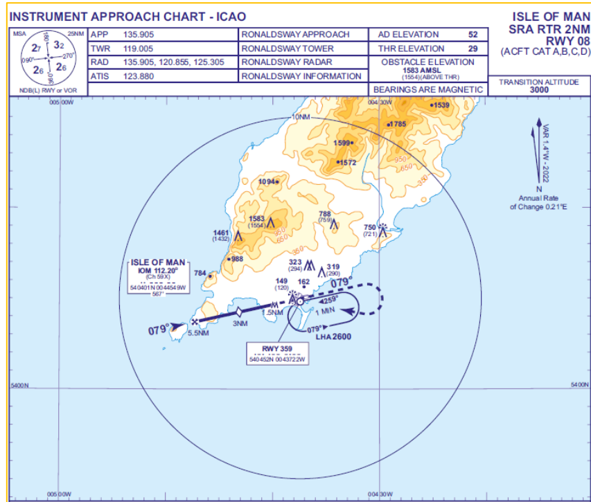
Figure 123 - SRA RWY 08
