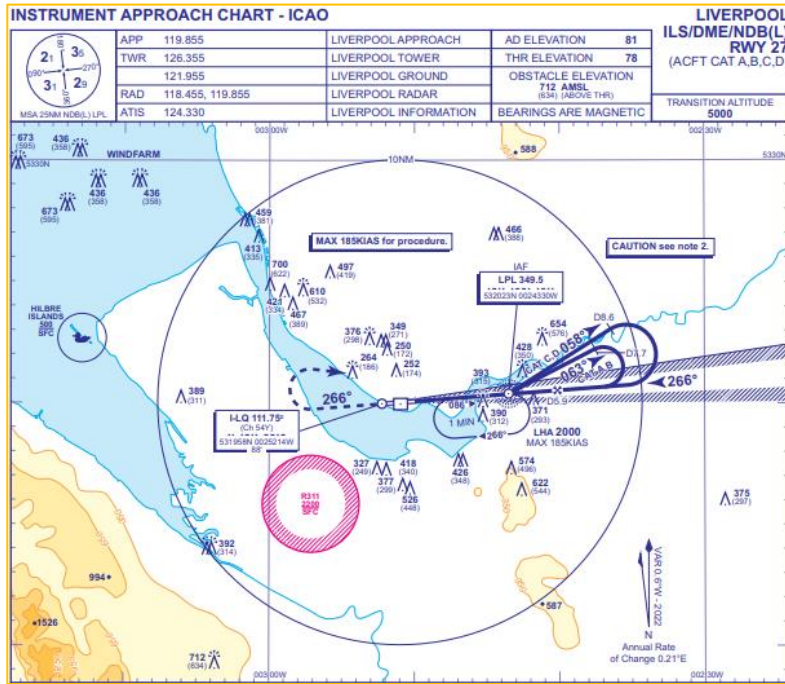
Figure 58 - ILS/DME/NDB(L) RWY 27 Procedure
