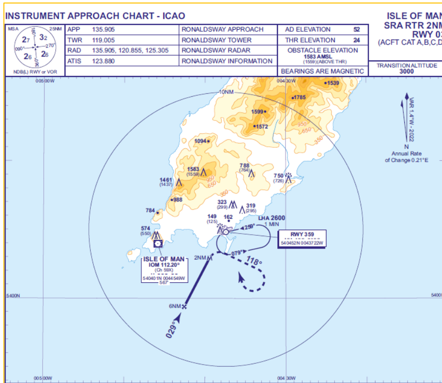
Figure 115 - SRA RWY03
