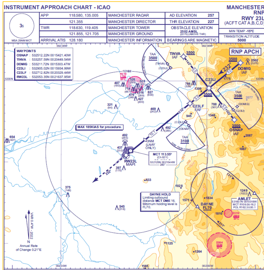
Figure 27 – RNP RWY 23L
