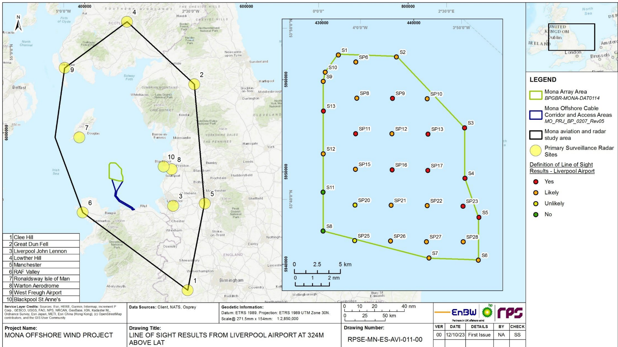
Figure 1.8: Liverpool Airport PSR LoS of the Mona Array Area (not to scale).
