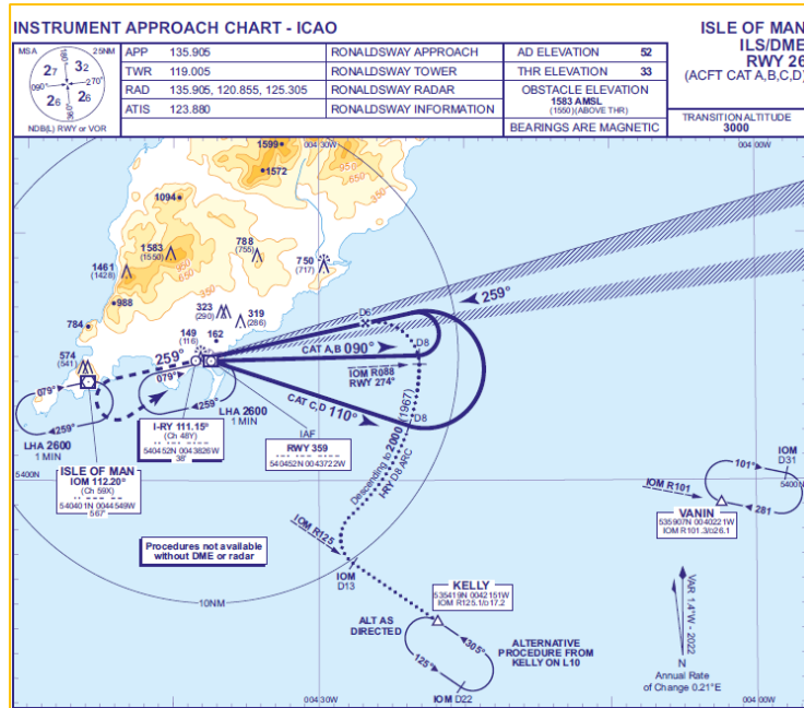
Figure 133 - ILS/DME RWY 26
