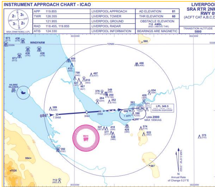
Figure 54 - SRA RTR 2NM RWY 09 Procedure
