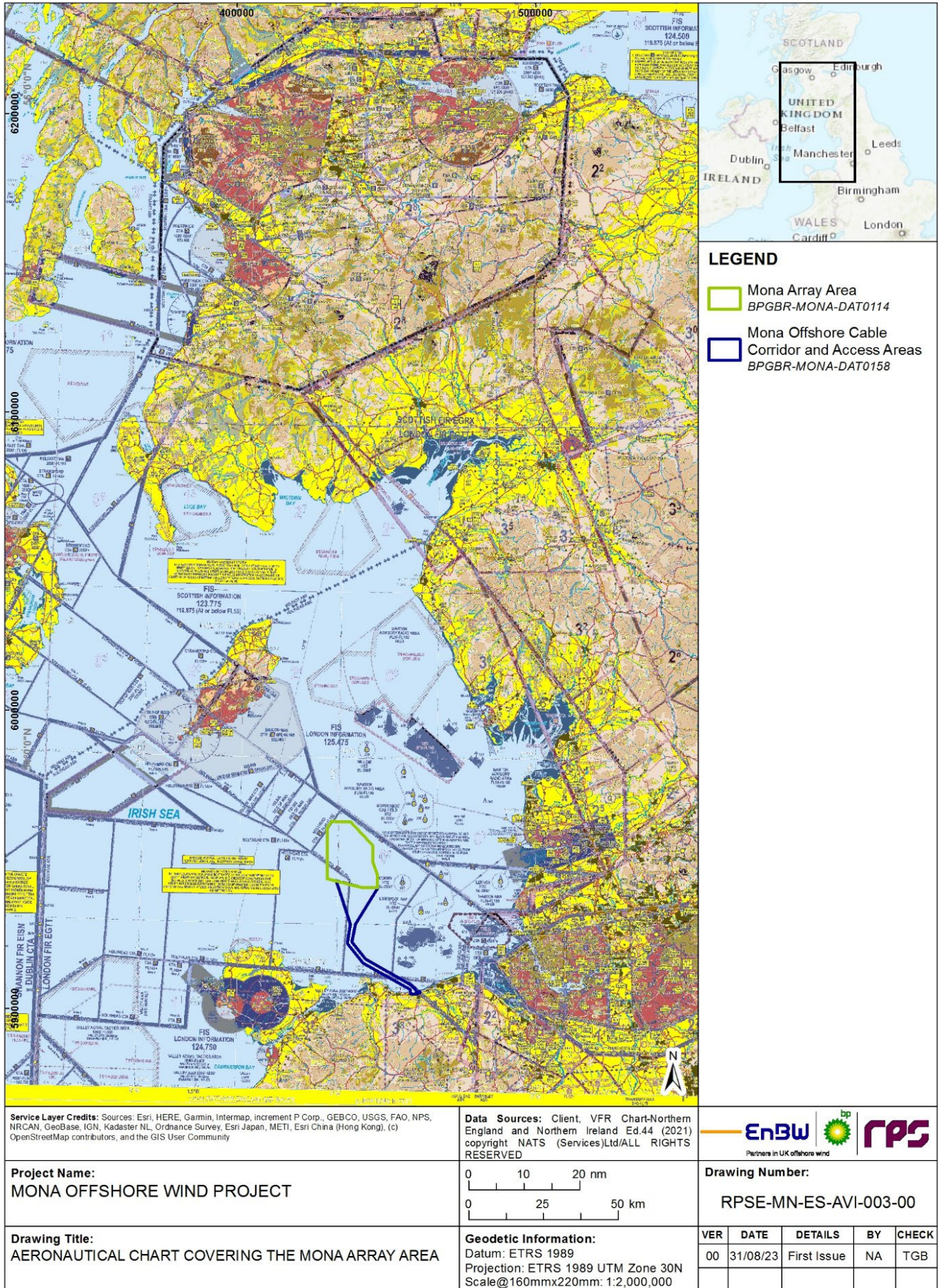
Figure 1.3: Airspace construct in the vicinity of the Mona Array Area.
