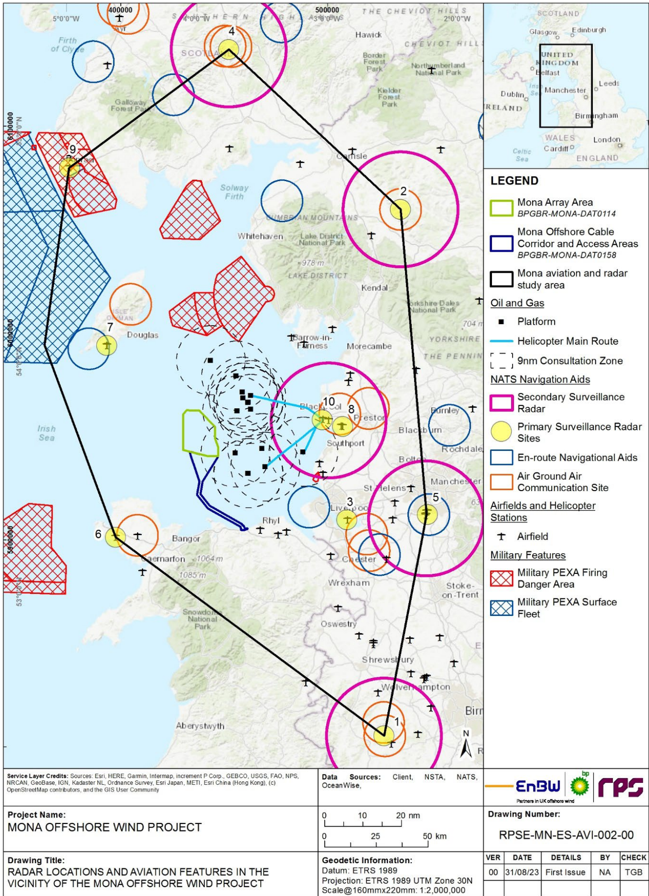
Figure 1.2: Radar locations and features within the vicinity of the Mona Offshore Wind Project.
