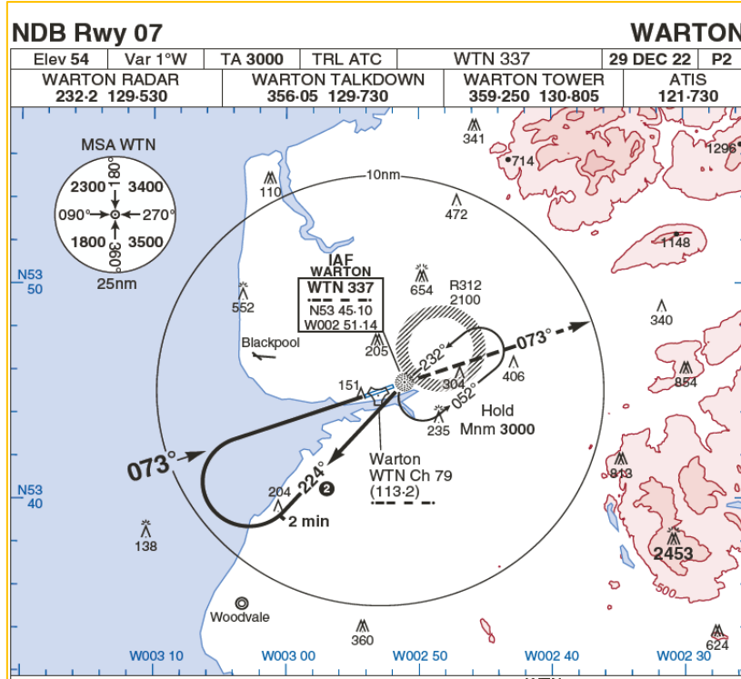
Figure 98 - NDB RWY 07 Procedure
